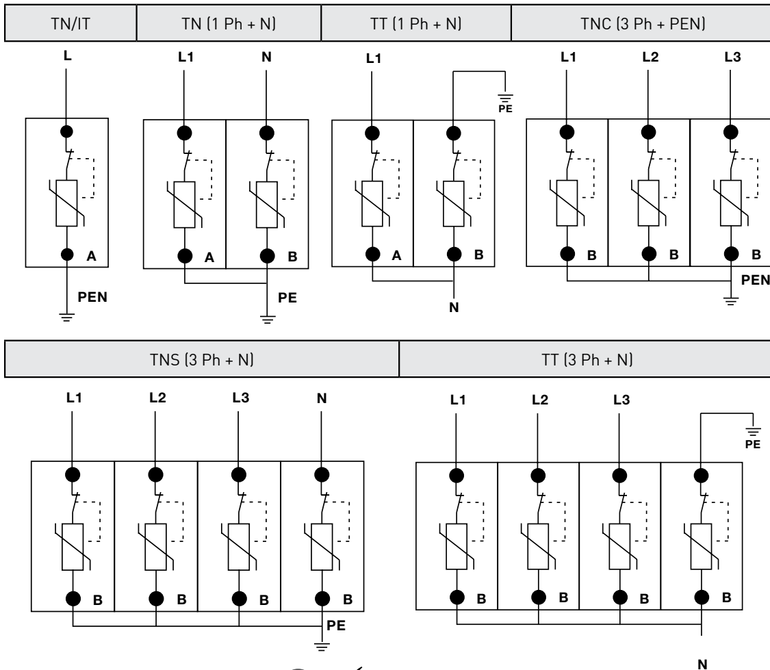
Figure 4 Wiring Diagram
