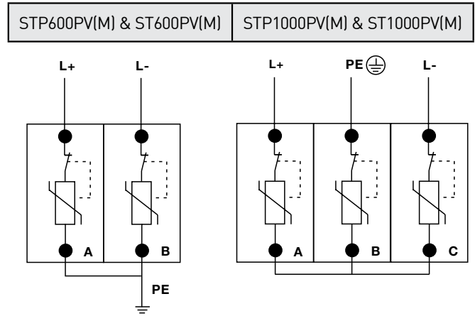
Wiring Diagram - Photovoltaic (PV)
