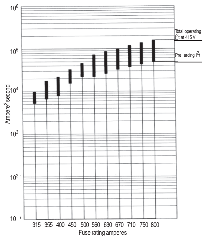
I^2t characteristics
